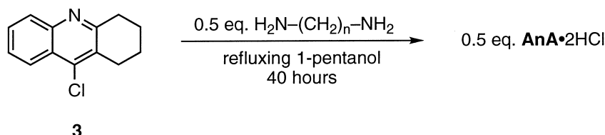
Scheme 2. Synthesis of THA dimers AnA by amination of 3 .
