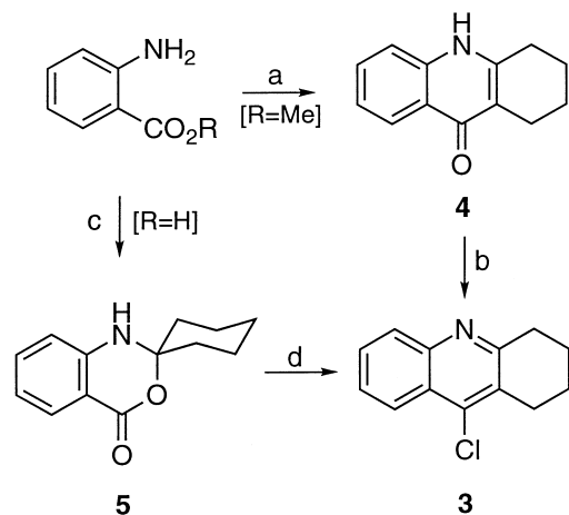
Scheme 3. Improved Synthesis of 3 . a) 1.2 equiv. cyclohexanone, 2.0 equiv. P_2O_5 , 2.0 equiv. N,N -dimethylcyclohexylamine, 170 °C (50%). b) 10 equiv. POCl_3 , reflux (85%). c) 1.2 equiv. cyclohexanone, toluene, Dean–Stark Trap, reflux (93%). d) 4 equiv. POCl_3 , reflux (96%).
