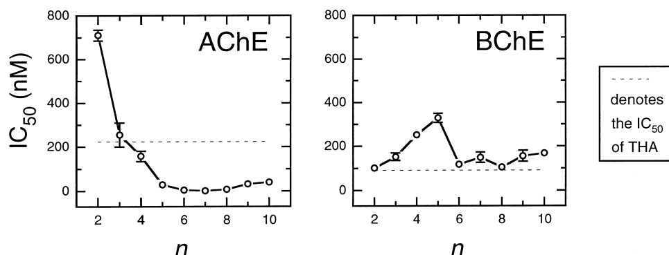
Figure 1. AChE and BChE inhibition by THA dimers AnA as a function of tether length n ( n =number of methylene units, IC_{50} values from Table 3). Where no error bars are shown, the error is smaller than the symbol.
