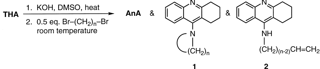
Scheme 1. Synthesis of THA dimers AnA by alkylation of THA .
